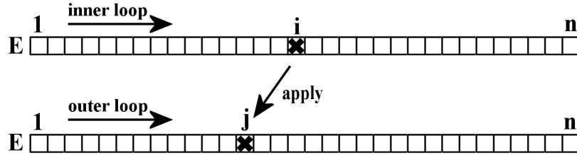
Figure 4: Selecting equations to apply LRBS
